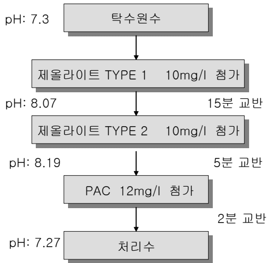
Fig.8 Water Treatment Process using Natural Zeolites
