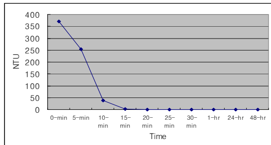
Fig.10 Variation of NTU due to Time
