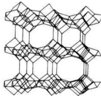
Clinoptilolite Structure
